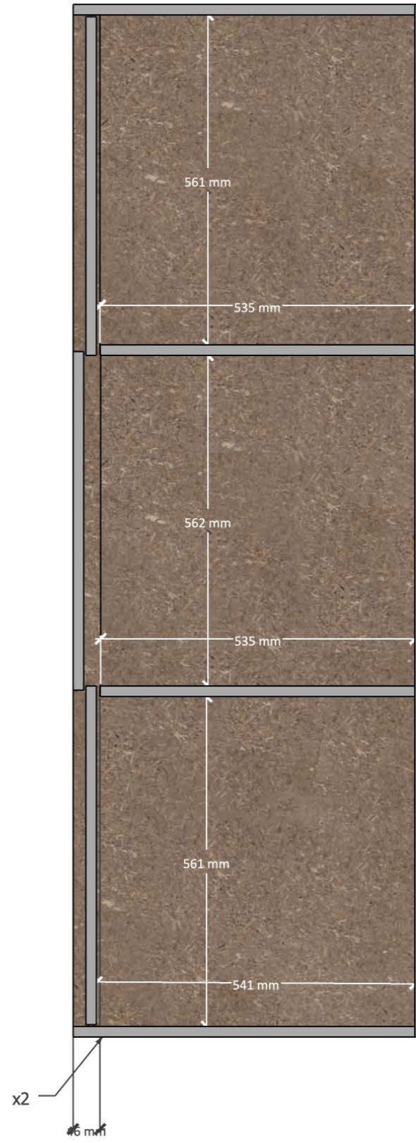
DB_sneede door corpus
